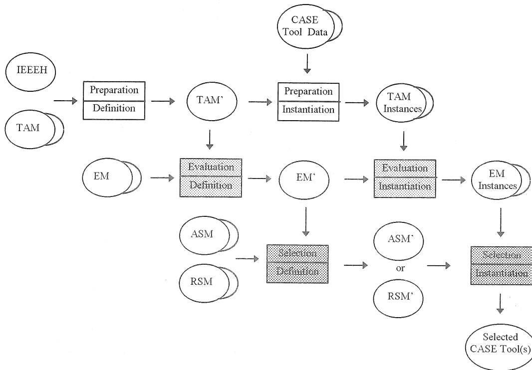
Figure 2 - Decision Process and Related Models
